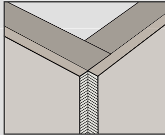
INNER CORNER JOINT
