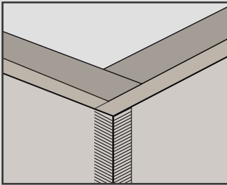
OUTER CORNER JOINT
